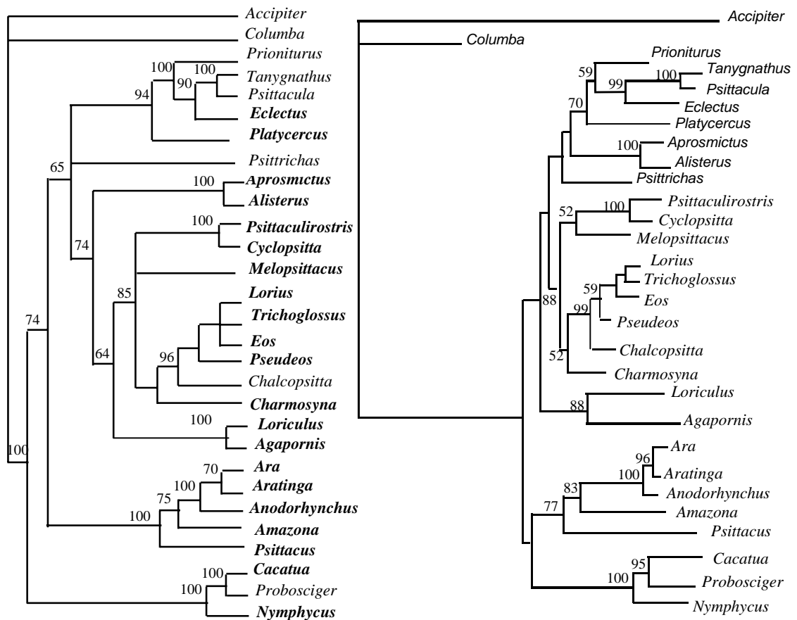
Fig. 1: Maximum-parsimony (left) and neighbor-joining (right) trees of parrots, based on sequence data of the seventh intron of the \beta -fibrinogen gene.
